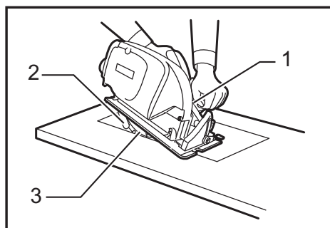
► 1. Retracting lever 2. Lower guard 3. Saw blade
