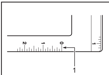
► 1. Position of blade edge when depth of cut is set at the deepest position
